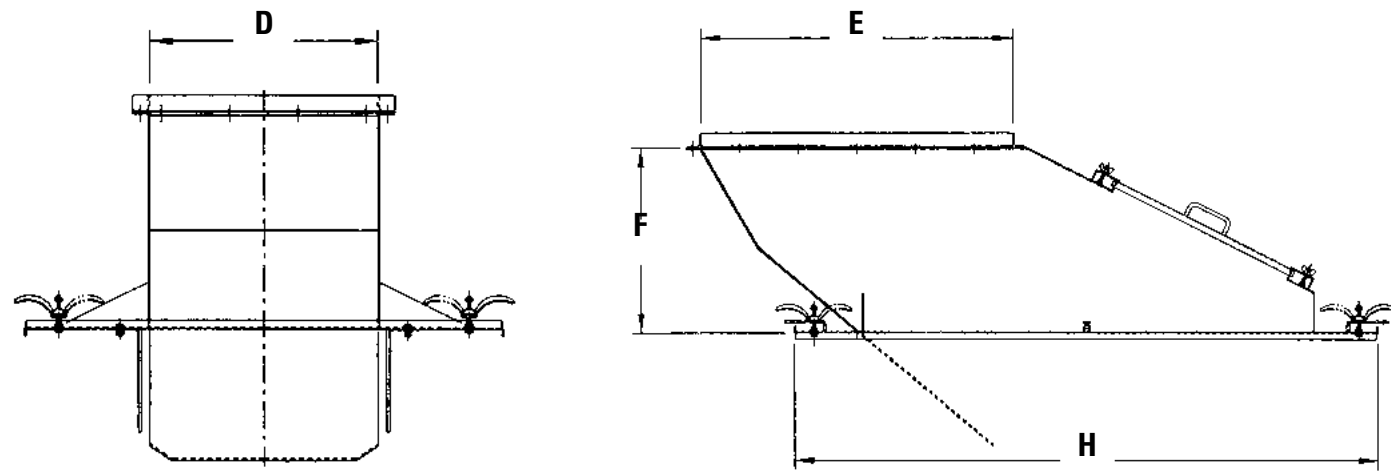
Above Typical initial inlet with fixed skirts Below Typical cleanout inlet with swing-down skirts
