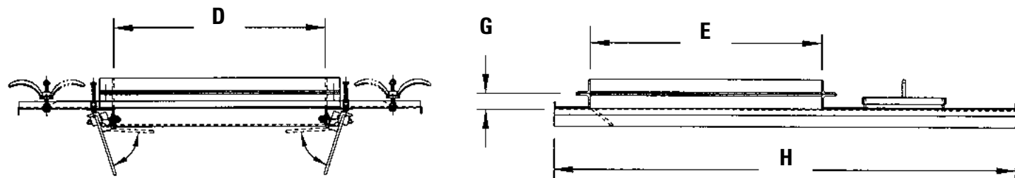
Above Typical initial inlet with fixed skirts Below Typical cleanout inlet with swing-down skirts
