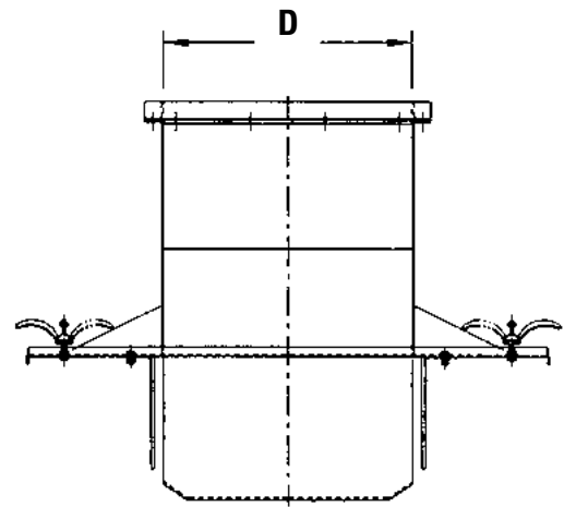
Above Typical initial inlet with fixed skirts
